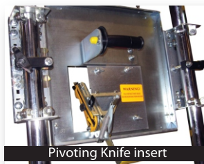
Makita Saw on a Spinning Insert w/Dust Collection
